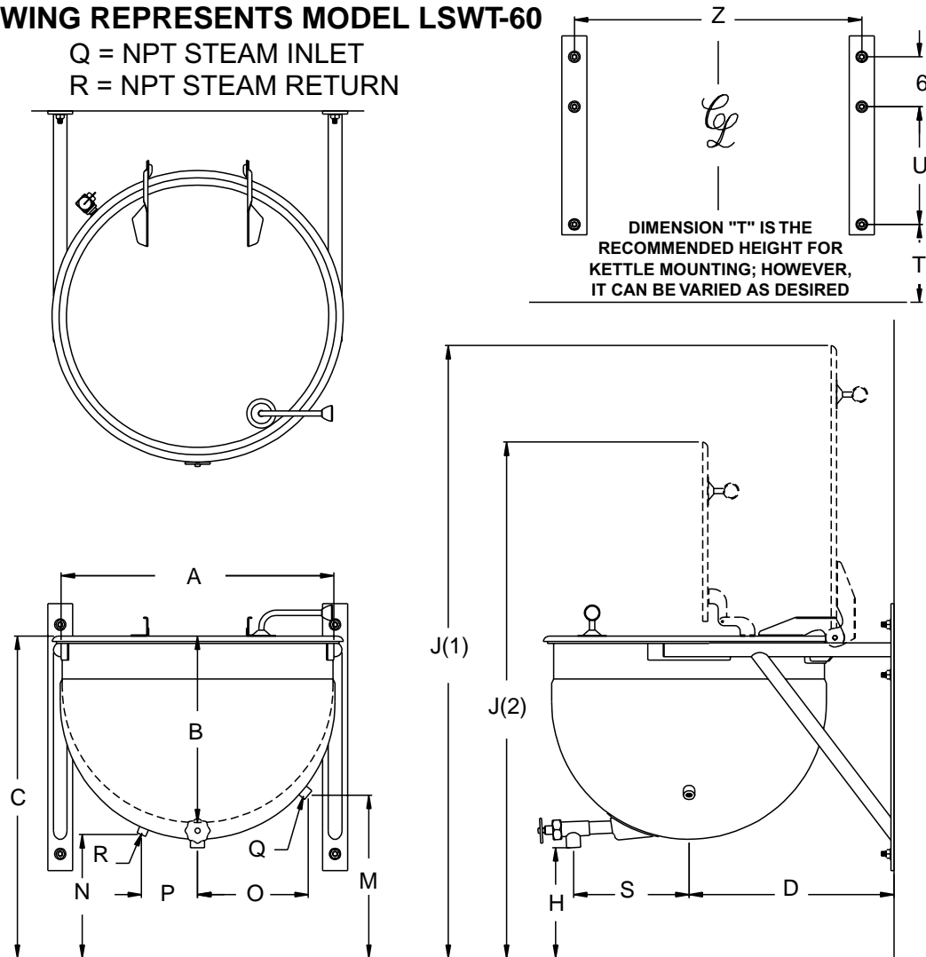
MODEL LSWT DIMENSIONS
