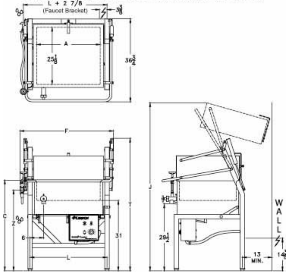
DRAWING REPRESENTS MODEL SKL6-9 WITH STANDARD 1 1/2 DRAW-OFF
